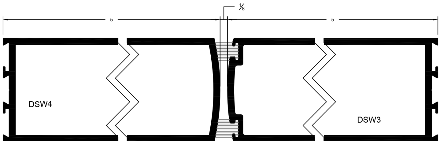
Meeting For Center / Offset Double Door
