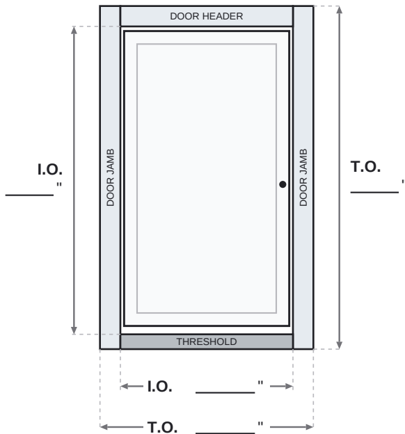
SINGLE DOOR
