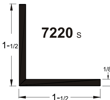
7220 S Equal Angle 1-1/2" x 1-1/2" 6' or 12'
