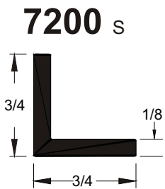
7200 S Equal Angle 3/4" x 3/4" 6' or 12'
