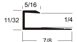
7830 BA 1/4" Coving Cap 8'
