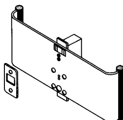
Pocket door pull. Standard model for walls 6" thick. 1069 is passage only non-latching comes with black nylon handles. ADA compliant
