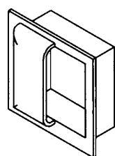
Size: 6" x 6" Depth: 1-1/2" BHMA: J403 Flush pull - Anti Vandal Meets California access requirements ADA compliant
