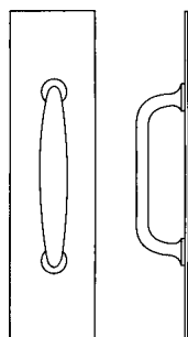
1010-3 Size: 4 x 16 BHMA: J405 CTC: 5" ADA compliant
