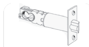
16-126 Dead Latch Square Corner 5" BS
