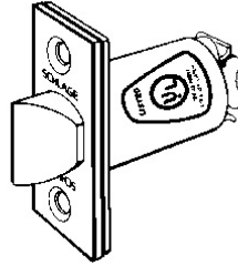
LATCH 13-048 Spring Latch Dimension: 1-1/8" x 2-1/4" square corner 1/2" throw 2-3/4 Backset
