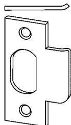
10-001 Square corner T Strike 1-1/8" x 2-3/4"
